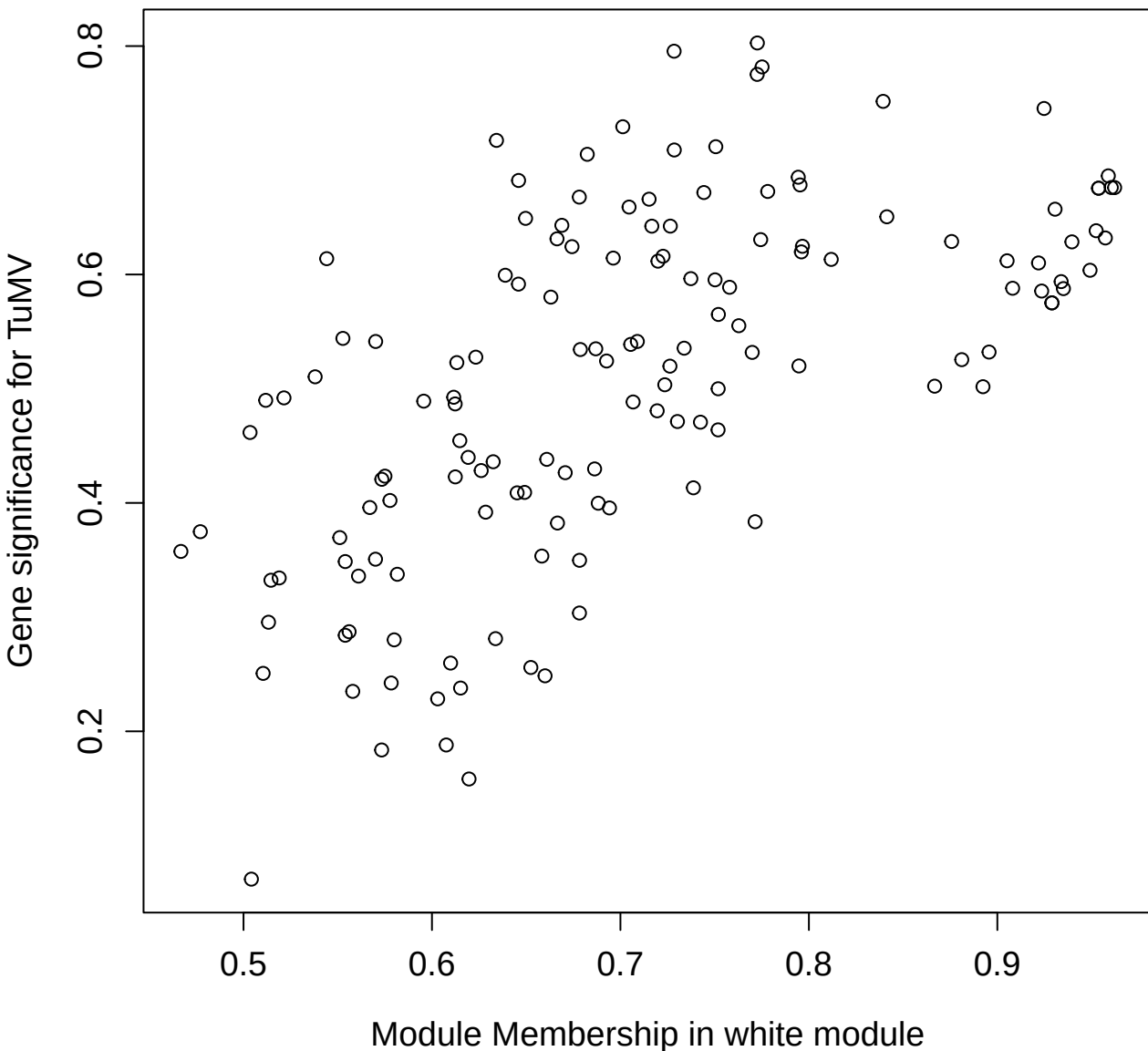
Module membership vs. gene significance cor=0.61, p=9.8e-16
